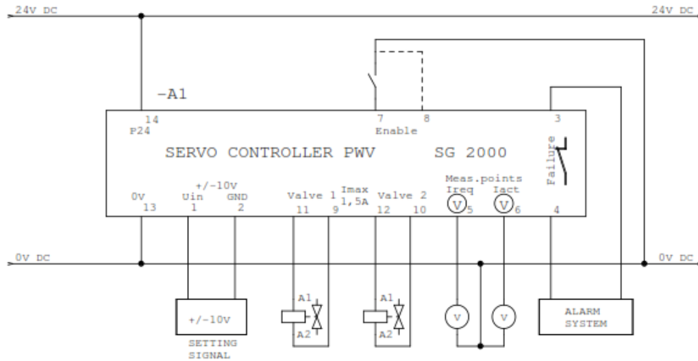
Fig. 1 principal scheme
